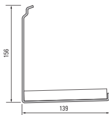
Regalboden 928 431 Shelf base 928 431
