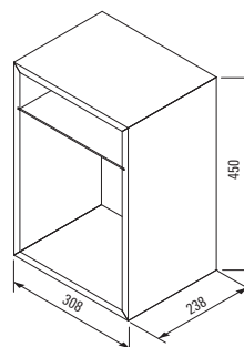
Box, offen 928 411 Box, open 928 411
