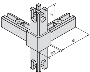
Eckknoten 4s 565 356 Corner joints, 4-sided 565 356
