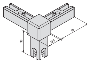
Eckknoten 3s 565 346 Corner joint, 3-sided 565 346
