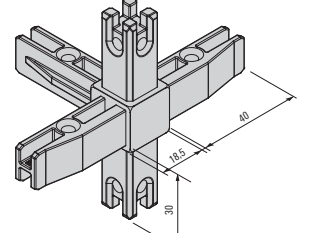
Eckknoten 5s 565 376 Corner joint, 5-sided 565 376
