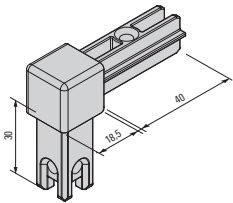
Eckknoten 2s 565 326 Corner joint, 2-sided 565 326
