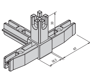
Eckknoten 4sh 565 366 Corner joint, 4-sided, horizontal 565 366
