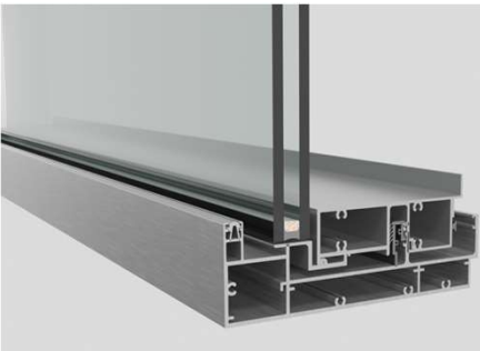
Typical bottom detail
