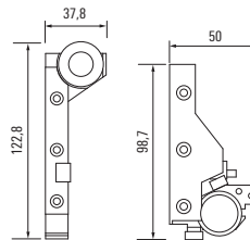
Slide Line M, fittings set not damped 100002692
