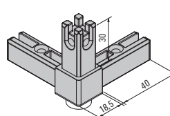
Corner joints 3 S including adjustable foot 100003070 E6/stainless steel 100003069 E6/C35 black
