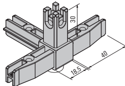
Corner joints 4 S H including adjustable foot 100003073 E6/stainless steel 100003072 E6/C35 black
