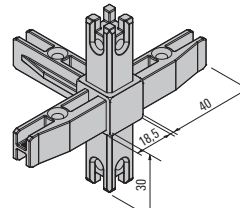
Corner joints 5 S 100003067 E6/stainless steel 100003066 E6/C35 black
