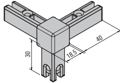
Corner joints 3 S 100003050 E6/stainless steel 100003049 E6/C35 black
