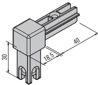
Corner joints 2 S 100003040 E6/stainless steel 100003039 E6/C35 black
