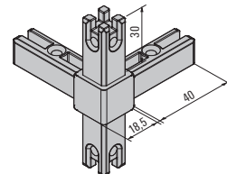
Corner joints 4 S 100003056 E6/stainless steel 100003055 E6/C35 black
