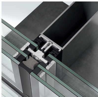
AOC 50 ST.SI SG (Structural Glazing)
