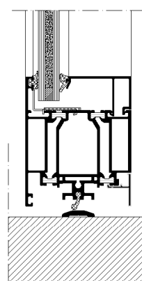
* Bunndetalj slepelist, skala 1:4
