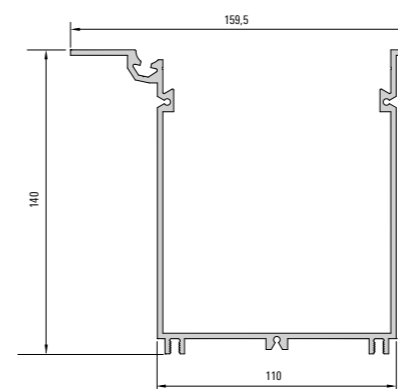
928 151 Cubeta
