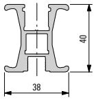
008317 Handle profile C
