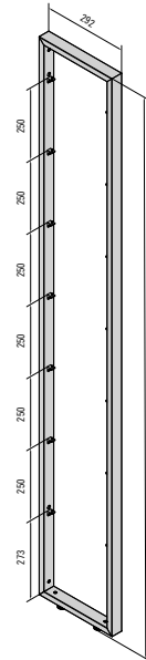
912 410 Frame 1950 mm
