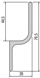
006773 Profile for corner carousel cabinet
