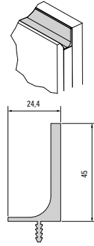
005805 Profile
