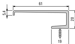
008233 Cover profile
