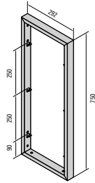
912 408 Frame 750 mm
