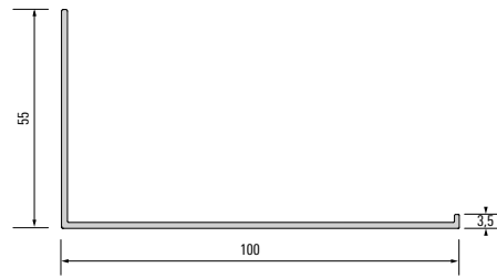
008447 Divider profile
