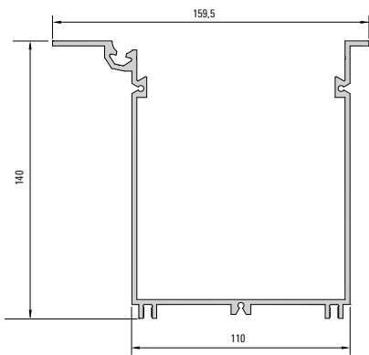
008558 Trough
