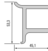
007428 Base support profile 25 mm
