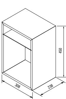
928 411 Box, open
