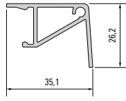
008543 Cover
