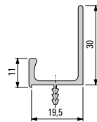
005192 Profile
