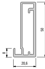
923 051 Profile
