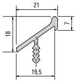
004699 Ladeo profile
