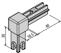
565 326 Corner joint, 2-sided
