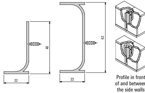
004117 Profile
