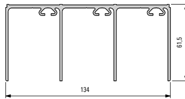
008340 Guide track, triple
