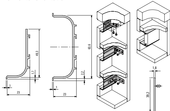
004264 Profile
