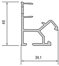
008534 Hanging rail
