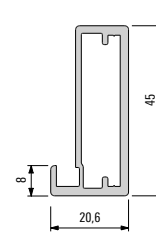
004512 Profile
