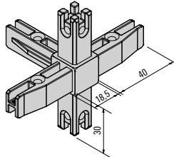
565 376 Corner joint, 5-sided
