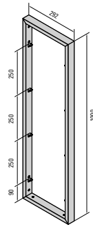
912 409 Frame 1000 mm
