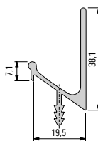
005156 Profile
