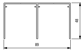
008387 Guide track, double
