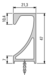
005317 Profile for 19 mm front depth
