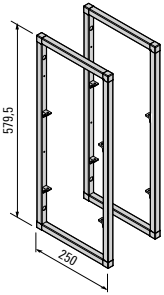
928 515 Kit for 580 mm side component
