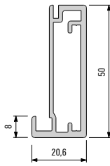
008123 Profile
