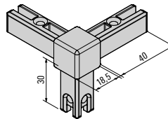
565 346 Corner joint, 3-sided
