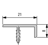
005030 Profile
