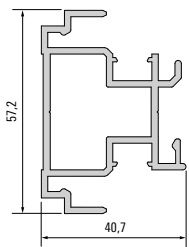
008569 Base support
