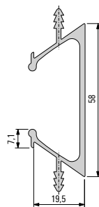
005185 Profile
