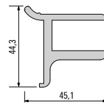
007057 Support profile for 16 mm base
