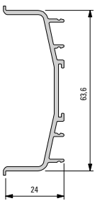
921 126 Profile
