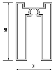
008683 Frame under roller fitting
