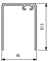
008353 Guide track, single
