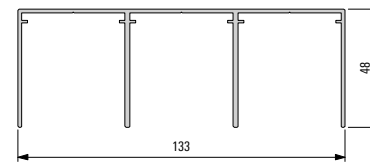
008393 Guide track, triple
