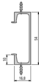
004678 Profile
