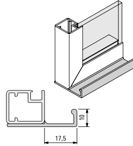
005123 Pull grip
