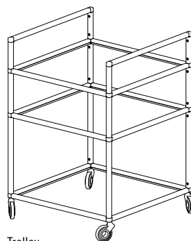
Trolley
