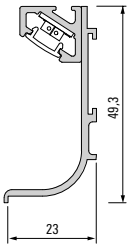
006773 Profile for corner carousel cabinet
