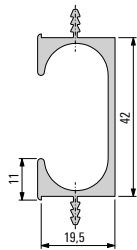
004063 Profile
