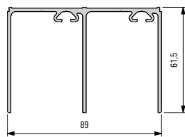
008350 Guide track, double
