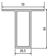
007587 Centre cross beam
