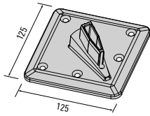
565 466 Bracket
