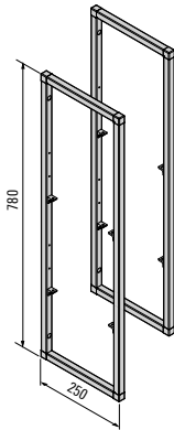
928 623 Kit for 780 mm side component
