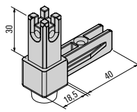
565 406 Corner joint, 2-sided, with adjustable foot
