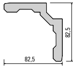
928 438 Corner cleat
