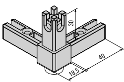
565 386 Corner joint, 3-sided, with adjustable foot
