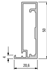
008192 Profile
