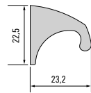
567 660 Denza profile
