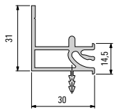
928 081 Profile
