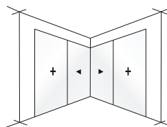
2D/1 90° innvendig ● 2D/1 90° inside
