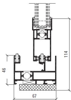
2-spors skyveparti
